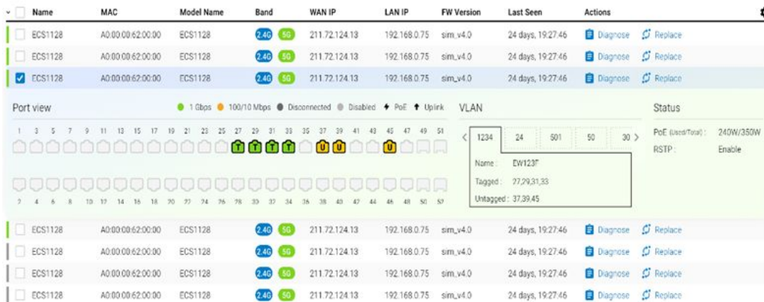
Figure 13- Switch device list view with quick dashboard
