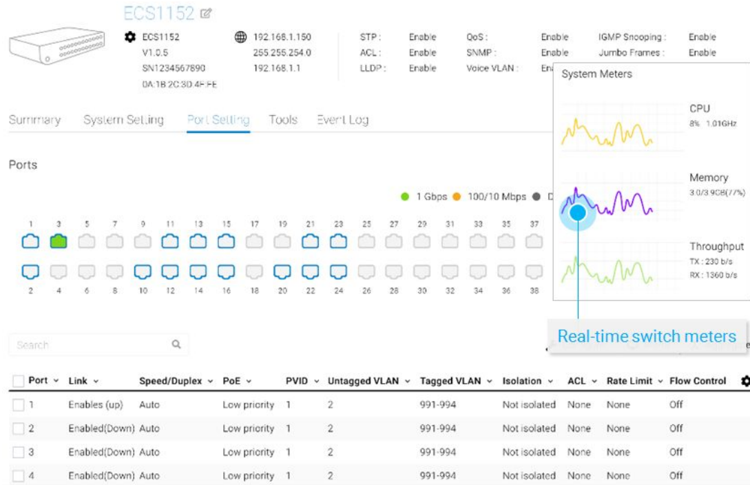
Figure 20 - Real-Time CPU and Memory of a switch
