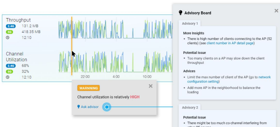
Figure 17- AI-Driven Advisor to lead the way to pinpoint real issues
